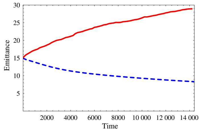
Figure 8. 95% normalized transverse emittance ( \mu\text{m} ) versus time (seconds) for Au ions and parameters of the RHIC-II upgrade, corresponding to figure 7. BETACOOOL simulations: solid (red) curve, emittance growth due to the IBS without cooling; dashed (blue) curve, emittance with cooling using rms dynamics approach.
